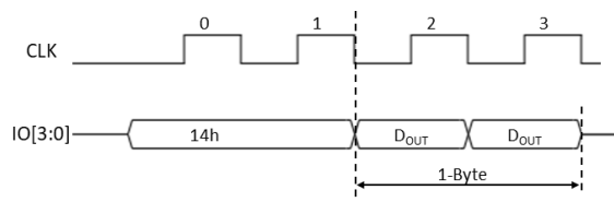
Figure 18: Read Any Register Timing
