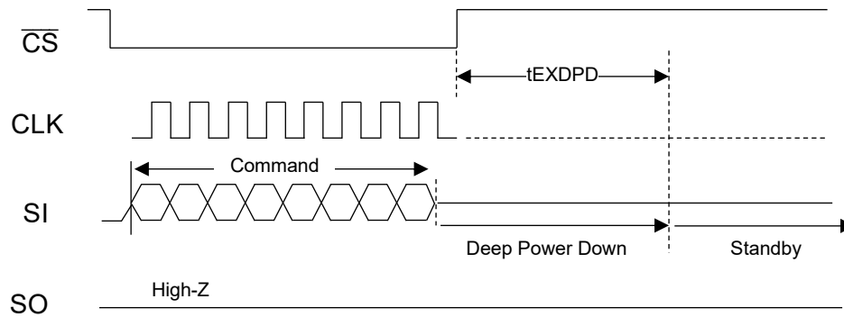
Figure 17 : Exit Deep Power Down Mode by SPI Command
