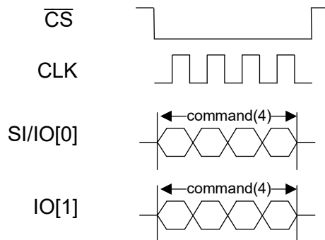
Figure 53 : Timing Description of 2-0-0 Instruction Type
