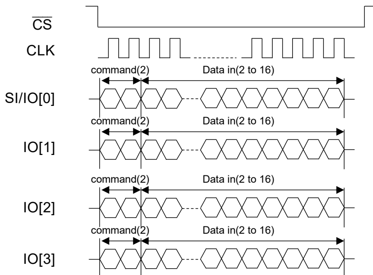
Figure 64 : Timing Description of 4-0-4 Instruction Type (Write)
