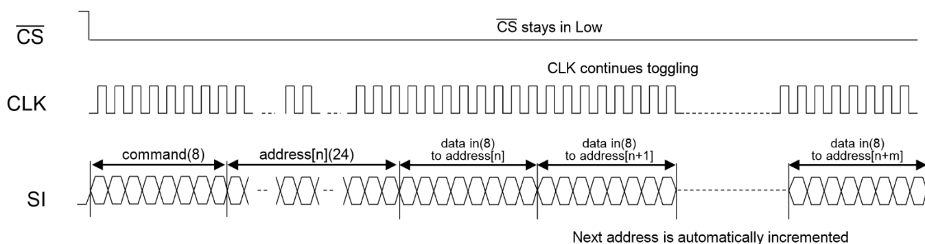
Figure 14 : Description of Continuing Write Operation (SSIP mode)
