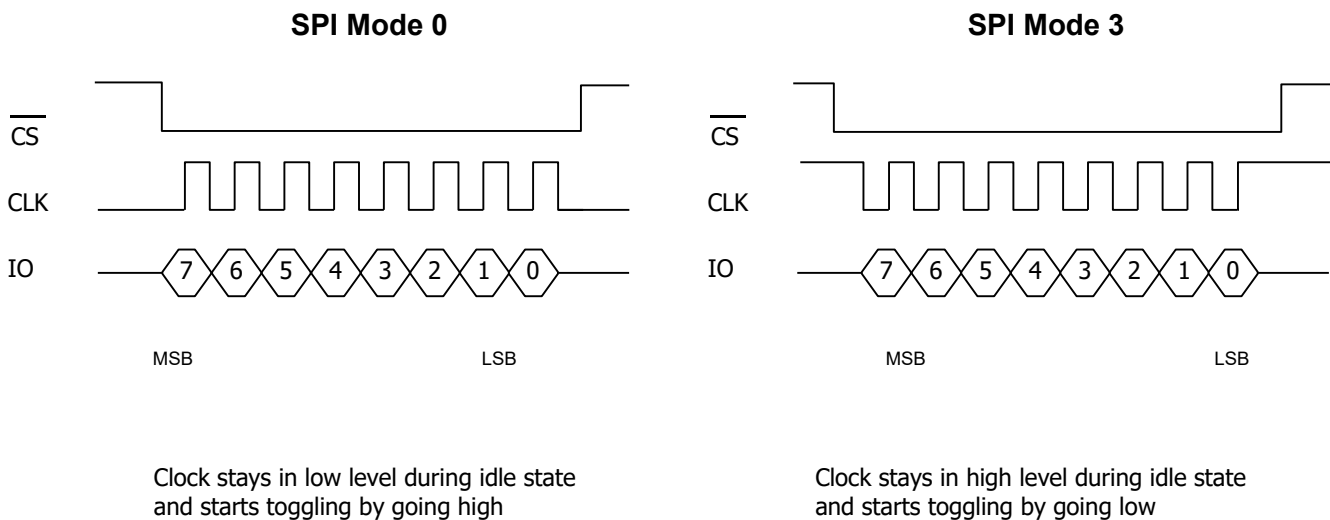
Figure 4 : SPI Clock Modes
