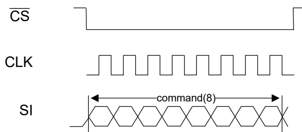
Figure 24 : Timing Description of 1-0-0 Instruction Type
