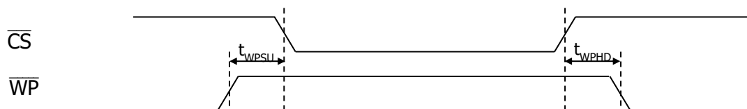
Figure 22 : \overline{WP} Operation Timing
