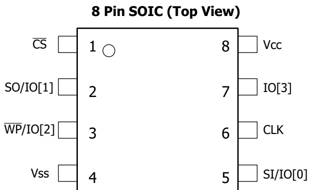
Figure 2 : Pinout
