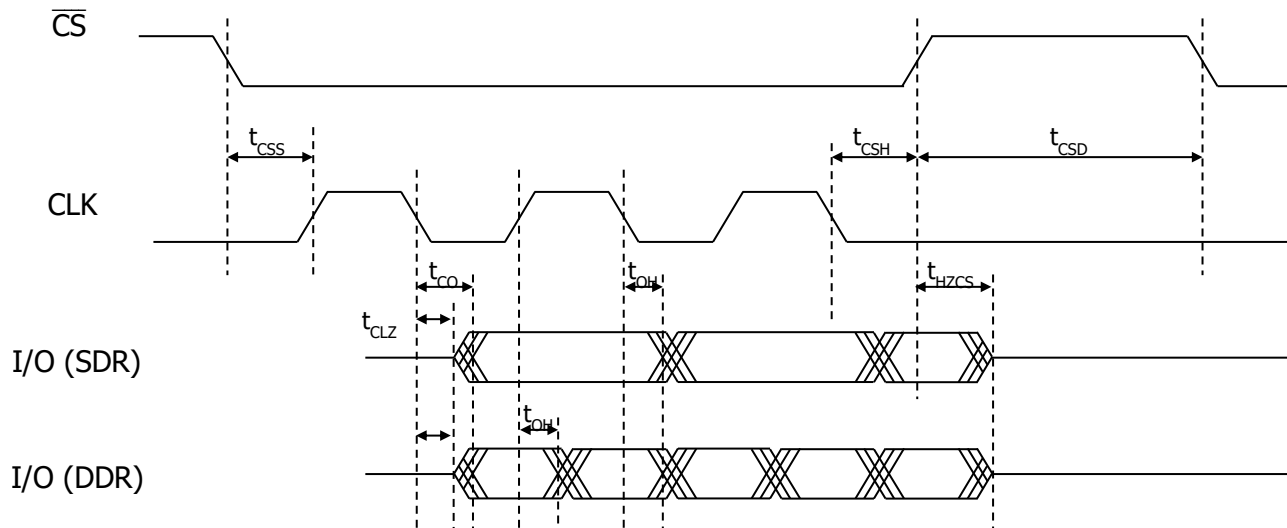
Figure 21 : Synchronous Data Output Timing (SDR/DDR)
