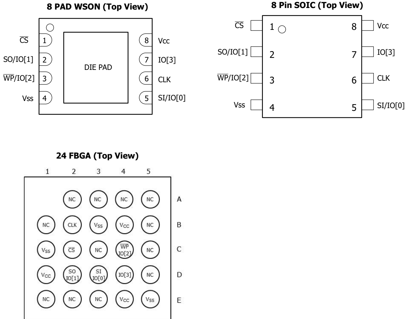
Figure 2 : Pinout
