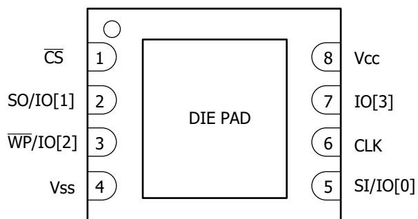
8 PAD WSON (Top View)
