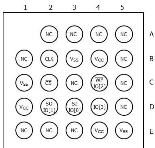
24 FBGA (Top View)
