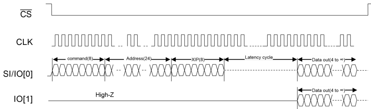
Figure 35 : Timing Description of 1-1-2 Instruction Type (Read with XIP)
